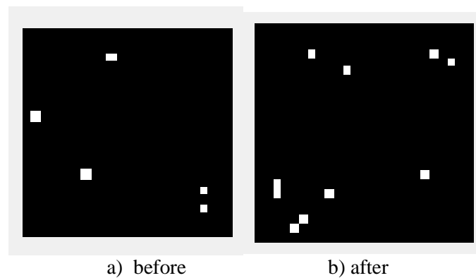
Figure 2: Placement of firms – creation
