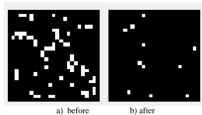
Figure 1: Placement of firms – extinction
